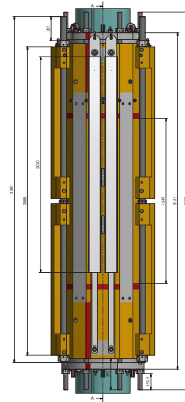
Conductor Repair Clamp Illustrative example
